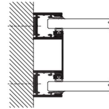
Wall connection
