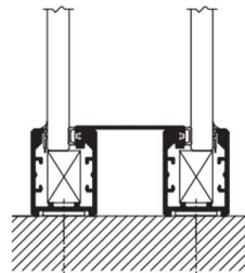
Ceiling connection
