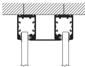
Floor connection
